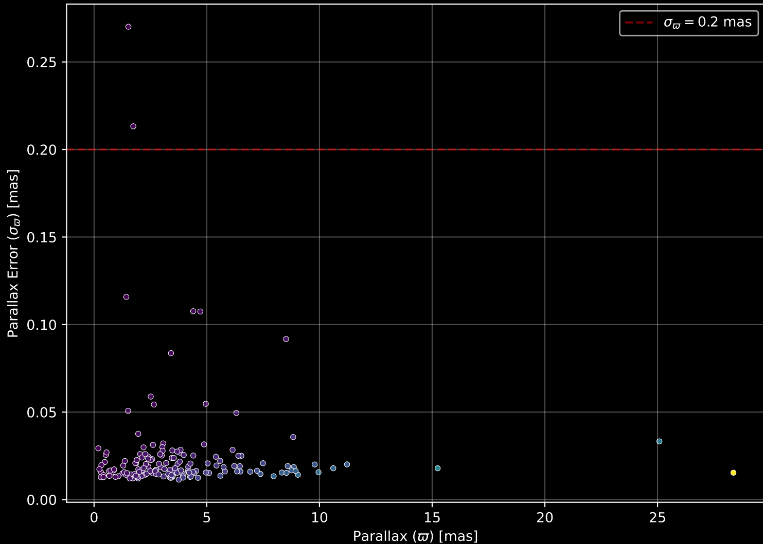
APOGEE DR17 Field: [103+81_MGA] Parallax Quality (n= 166)
