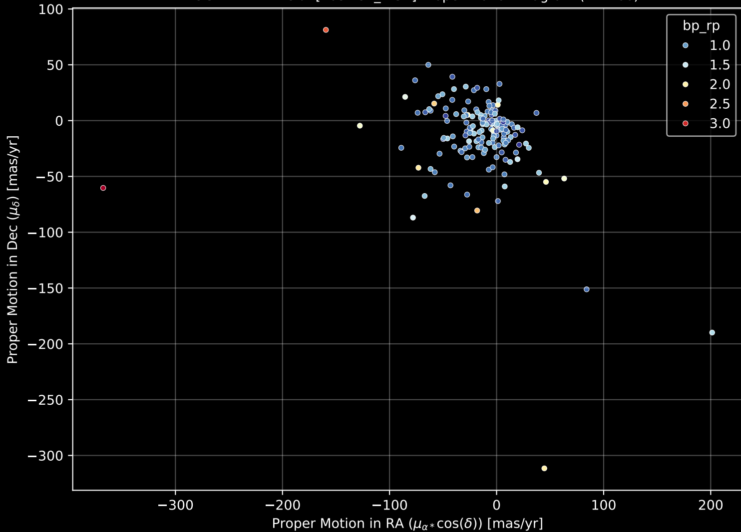
APOGEE DR17 Field: [103+81_MGA] Proper Motion Diagram (n= 166)
